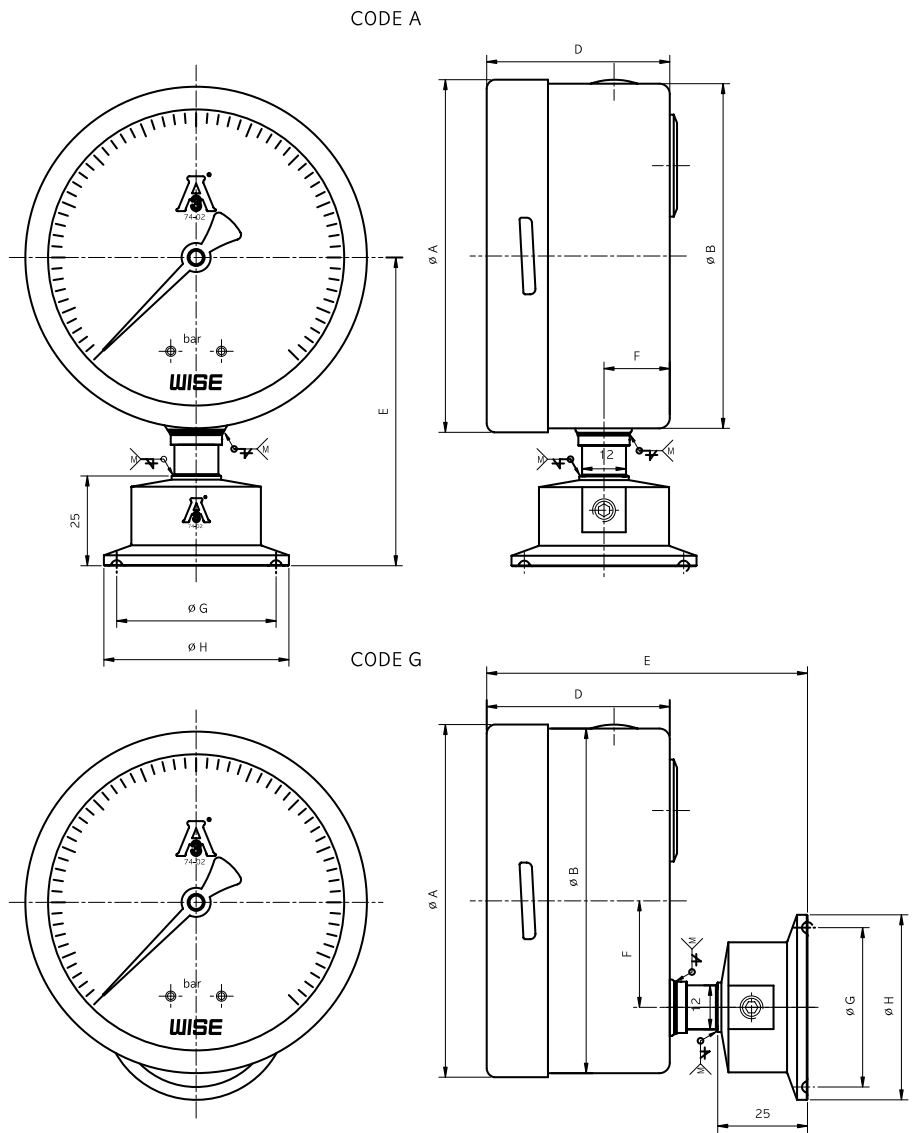
Dimensions (mm)
